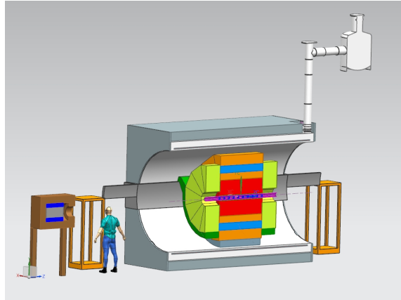
Figure 3: Schematic layout of REDTOP detector.
