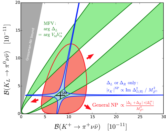
Figure 42: Scheme for BSM modifications of K \rightarrow \pi \nu \bar{\nu} BRs. Reproduced from Ref. [339].
