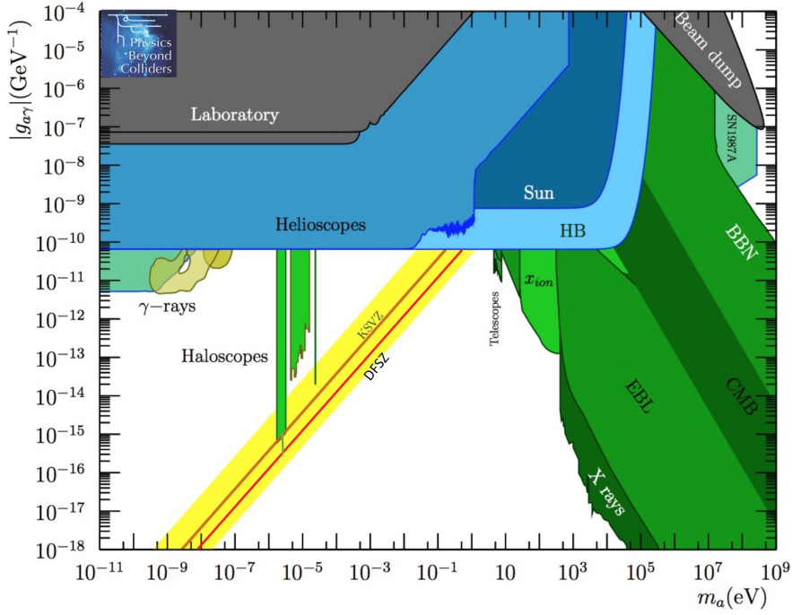
Figure 15: Current constraints for the axion photon coupling g_{a\gamma} versus axion mass m_a . Revised from [38]. See text for details.
