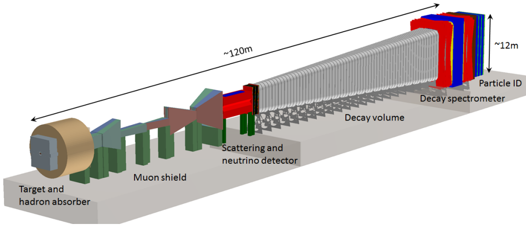
Figure 7: Layout of the SHiP detector.
