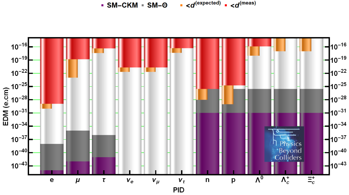
Figure 13: Overall status of EDM measurements: current limits on EDMs of fundamental particles are displayed as red bars from the top. From below come the SM estimates from CKM CP violation and \Theta_{QCD} . White regions indicate safe BSM discovery territory for the experiments.
