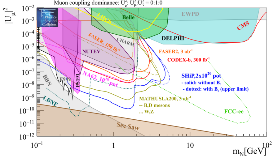
Figure 33: BC7: Sensitivity to Heavy Neutral Leptons with coupling to the second lepton generation only. Current bounds (filled areas) and 10-15 years prospects for PBC projects (SHiP, MATHUSLA200, CODEX-b and FASER2) (dotted and solid lines). Projections for the LBNE near detector with 5 \times 10^{21} pot and FCC-ee with 10^{12} Z^0 decays are also shown.
