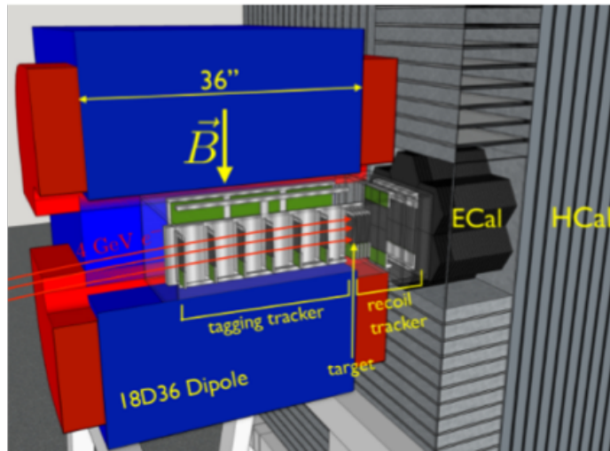
Figure 5: The LDMX experiment layout.
