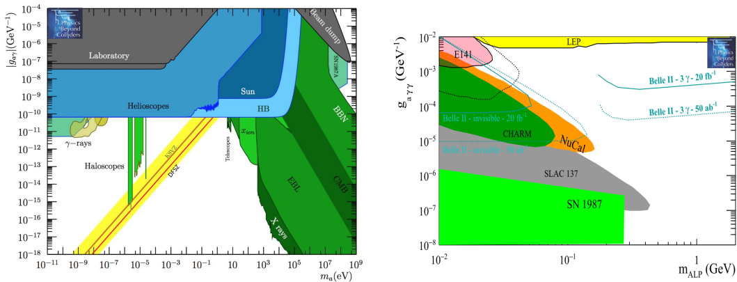
Figure 36: Left panel: current limits on axion with photon coupling in the plane coupling ( g_{a\gamma\gamma} ) versus mass ( m_a ). The right panel shows the zoom in the range of masses interesting for accelerator-based experiments (note the different units for the mass ranges in the two panels). In the left pane, current bounds are shown as filled coloured areas. A possible sensitivity from Belle-II from a phenomenological study [303] is also shown.
