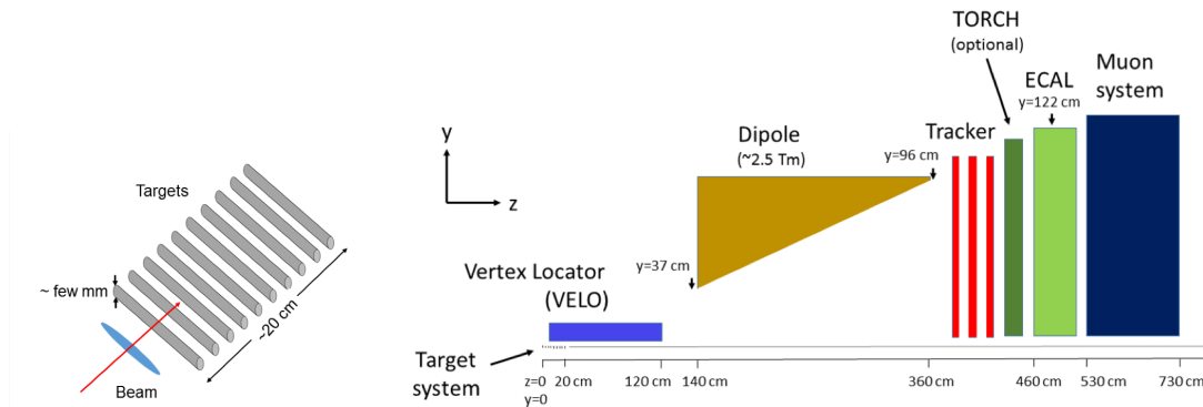
Figure 12: Schematic layout of the target system (left) and the spectrometer (right) of the TauFV experiment.
