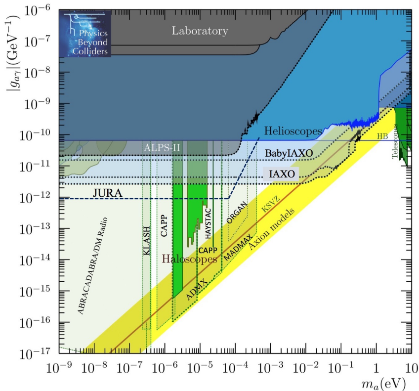
Figure 16: Physics reach of Baby-IAXO, IAXO and JURA compared with other experiments currently proposed and/or planned in the world. Revised from [38]. See text for details.
