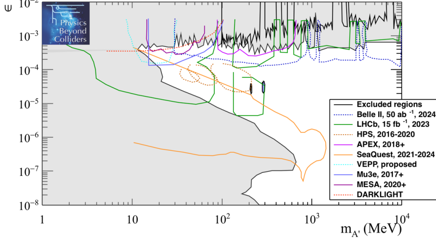
Figure 18: Future upper limits at 90 % CL for dark photon in visible decays in the plane mixing strength \epsilon versus mass m_{A'} from experiments and proposals not related to the PBC activity.
