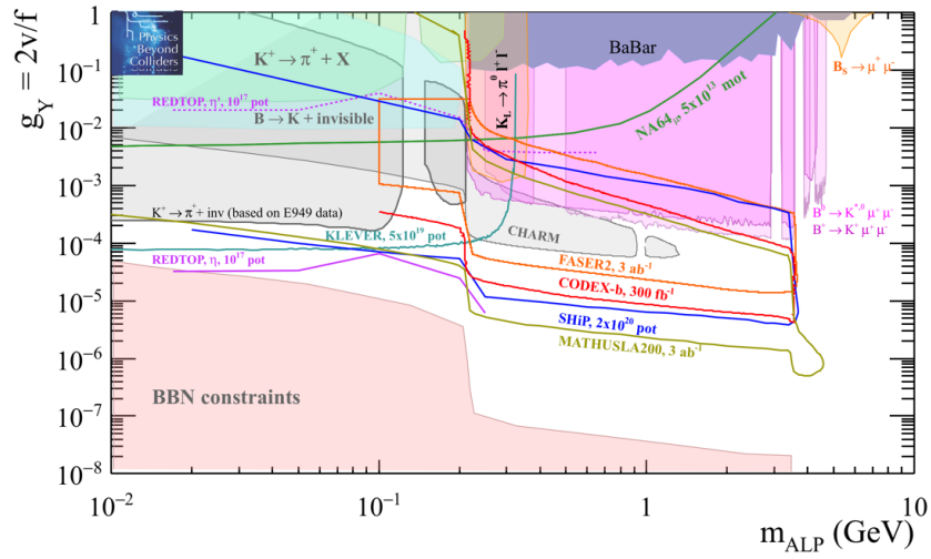
Figure 40: BC10: ALPs with fermion coupling. Current bounds (filled areas) and medium-far ( \sim 10 -15 years) prospects for PBC projects (solid lines) for ALPs with fermion coupling. CHARM and LHCb filled areas have been adapted to PBC prescriptions by F. Kahlhoefer, following Ref. [318]. E949 area has been computed by the KLEVER collaboration and M. Papucci based on E949 data. All other exclusion regions have been properly re-computed by M. Papucci, following Ref. [317].
