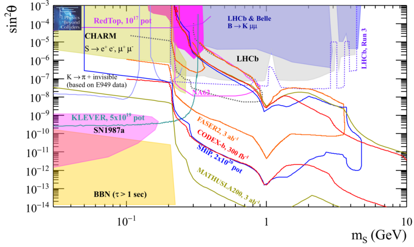
Figure 29: BC5: prospects on 10-15 year timescale for PBC projects for the dark scalar mixing with the Higgs in the plane mixing angle \sin^2 \theta versus dark scalar mass m_S under the hypothesis that both parameters \lambda and \mu are different from zero. The sensitivity curves have been obtained assuming BR(h \rightarrow SS) = 10^{-2} . The NA62 ++ and KLEVER curves correspond still to the case of \lambda = 0 , and, hence, should be considered conservative.
