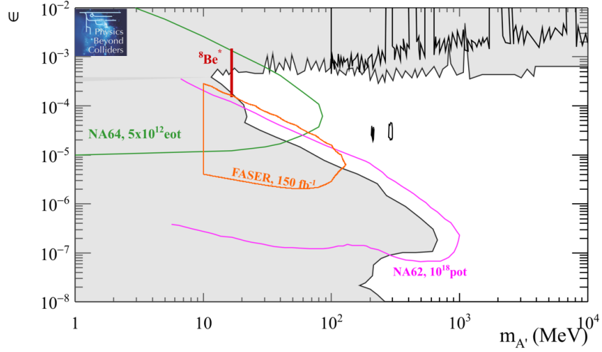
Figure 19: PBC projects on \sim 5 year timescale: upper limits at 90 % CL for Dark Photon in visible decays in the plane mixing strength \epsilon versus mass m_{A'} . The vertical red line shows the allowed range of e - X couplings of a new gauge boson X coupled to electrons that could explain the {}^8\text{Be} anomaly [70, 71].
