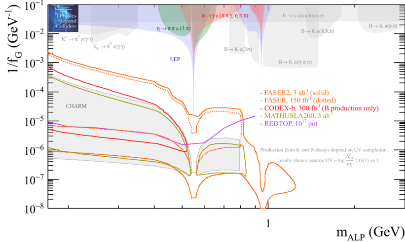
Figure 41: Current bounds (as coloured filled areas) and the prospects for PBC projects (solid lines) both on 5- (FASER) and 10-15 year (CODEX-b, MATHUSLA200, FASER2) timescale. The CHARM gray filled area has been computed by F. Kling, recasting the search for long-lived particles decaying to two photons performed at CHARM [195]. Other coloured filled areas are kindly provided by Mike Williams and revisited from Ref. [324]. The gray areas depend on UV completion and the results shown assume \approx [\log \Lambda_{UV}^2/m_t^2 \pm \mathcal{O}(1)] \Rightarrow 1 . The CODEX-b curve has been obtained considering B-decays only, hence it is conservative. Both NA62 ++ and SHiP are sensitive to this benchmark case too, the curves are currently being compiled.
