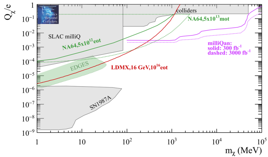
Figure 25: BC3: milli-charged particles. Current bounds (filled areas), experimental landscape and physics reach of PBC projects in 5 years time scale (NA64 ++ ( e ) and NA64 ++ ( \mu )), and in 10-15 years time scale (LDMX @ eSPS).
