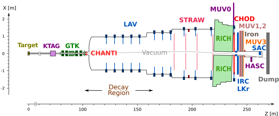
Figure 4: Layout of the NA62 experiment.
