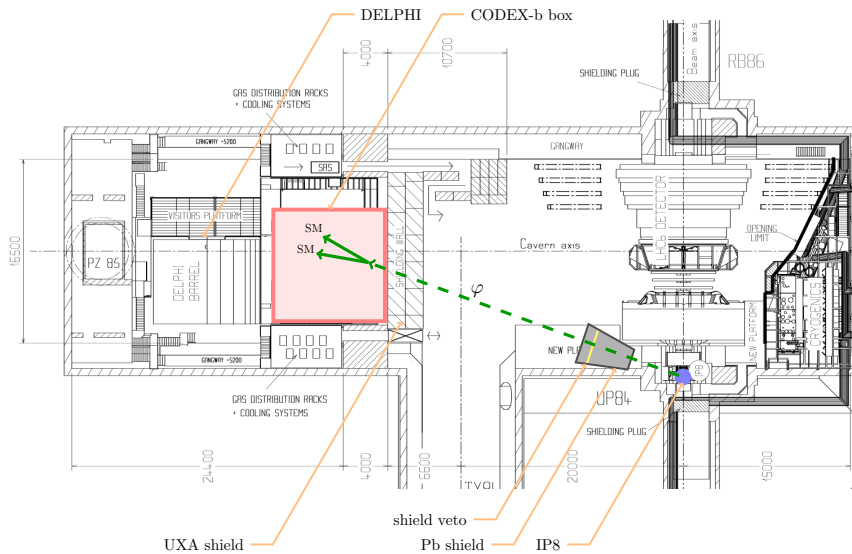
Figure 10: Layout of the LHCb experimental cavern UX85 at point 8 of the LHC [113], overlaid with the proposed CODEX-b location.
