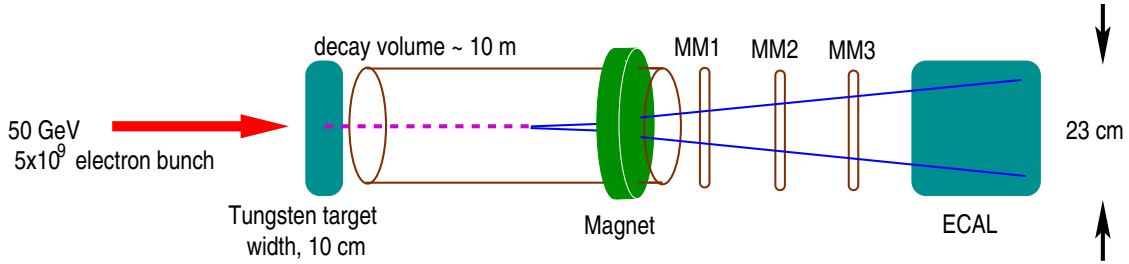
Figure 6: The AWAKE/NA64 conceptual layout.
